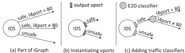
Figure 5: E2 converts edge annotations on an iGraph (a) into output vports (b) that the applications write to, and then adds traffic filters that the E2D implements (c).
